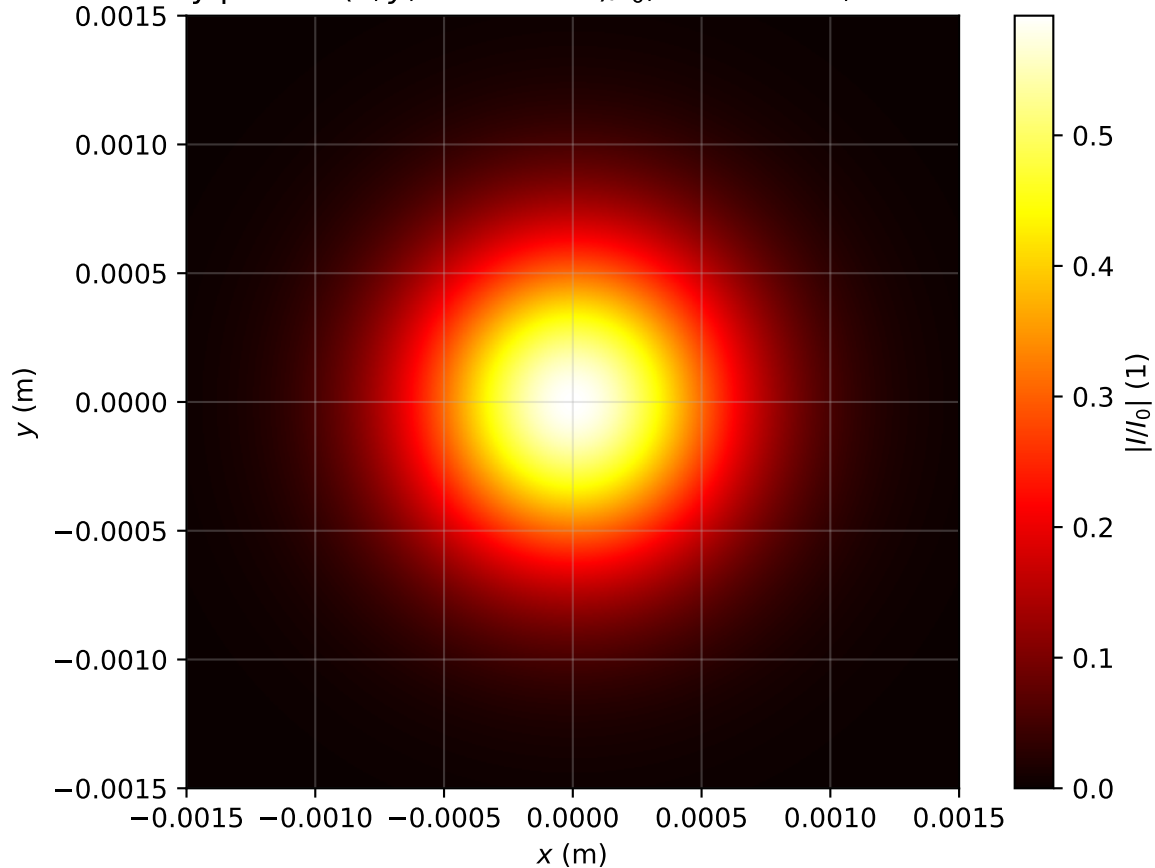
Intensity profile I(x, y, z = 2.229m)/I_0 , Pin=0.3Pcr, artificial time
